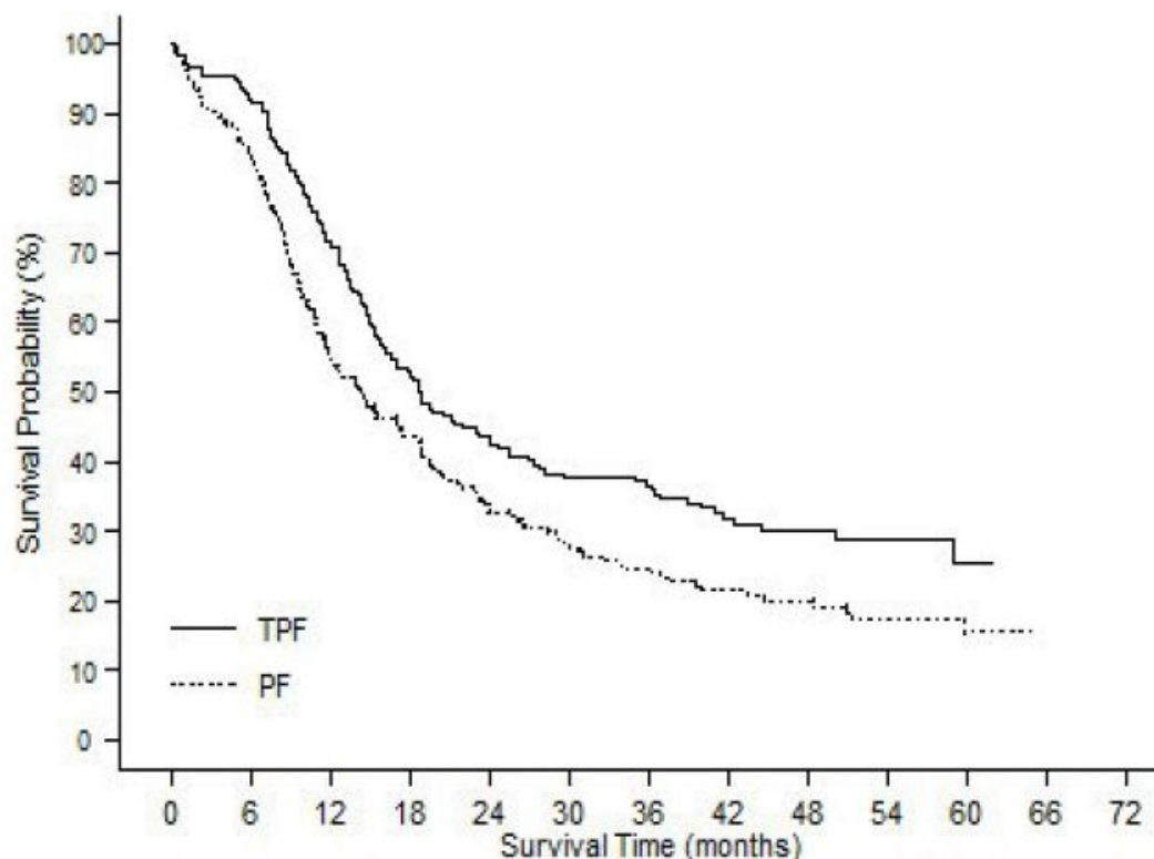
Figure 9: TAX323 Overall Survival K-M Curve
