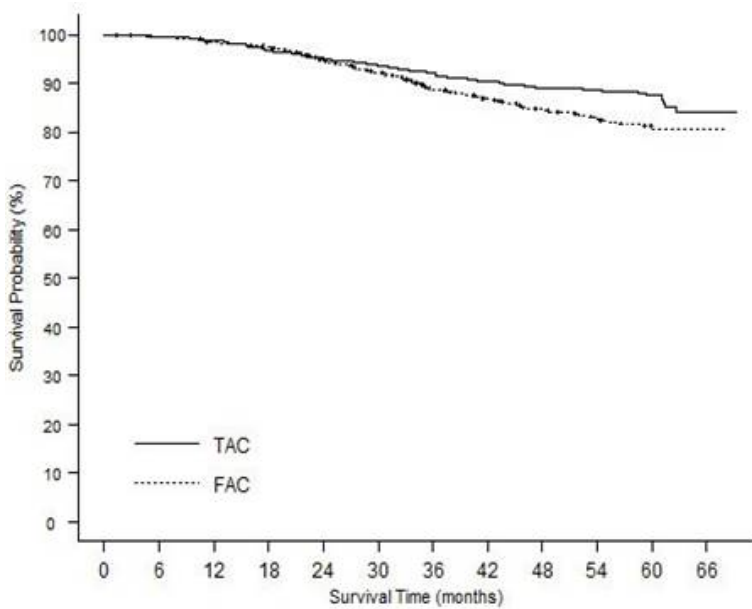
Figure 2: TAX316 Overall Survival K-M Curve
