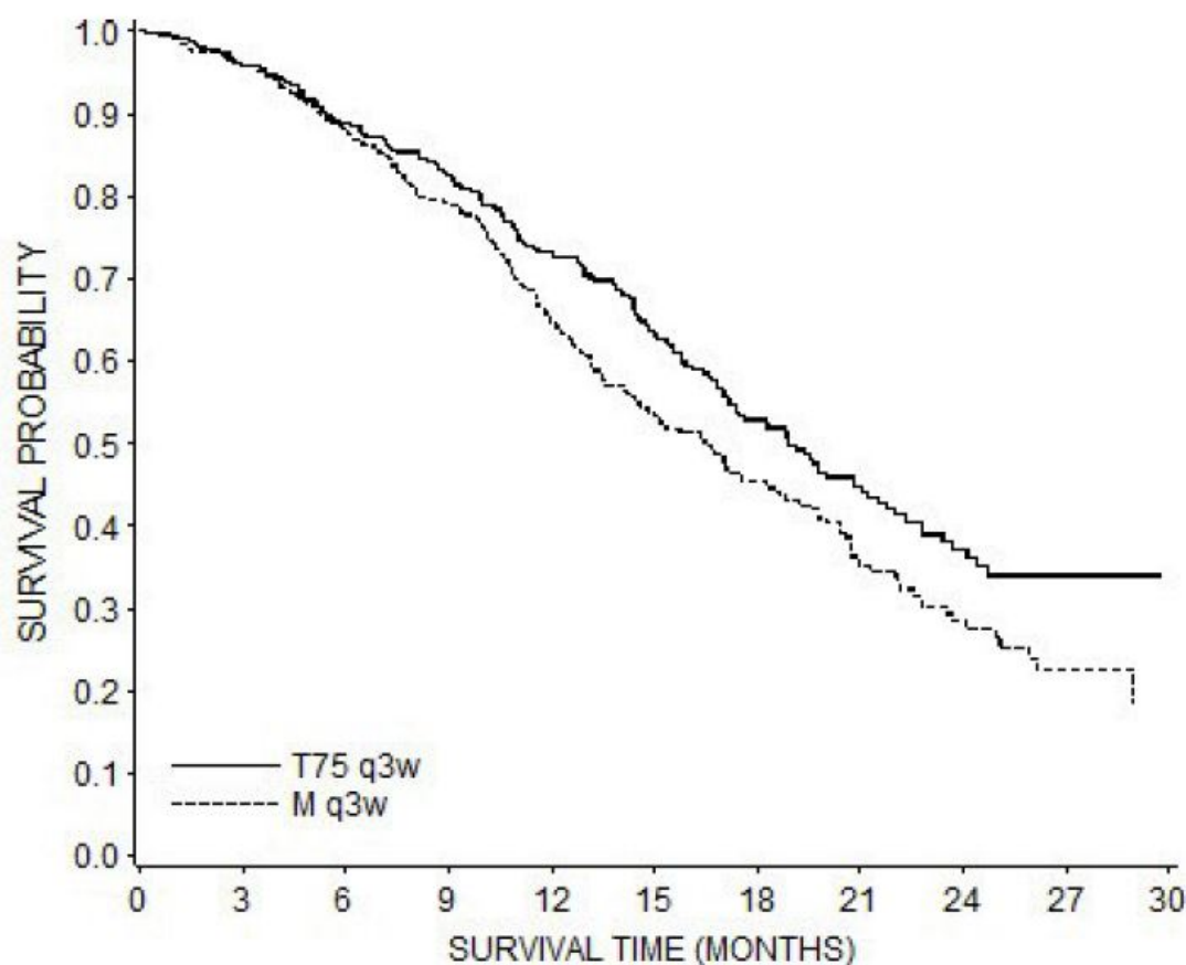
Figure 5: TAX327 Survival K-M Curves
