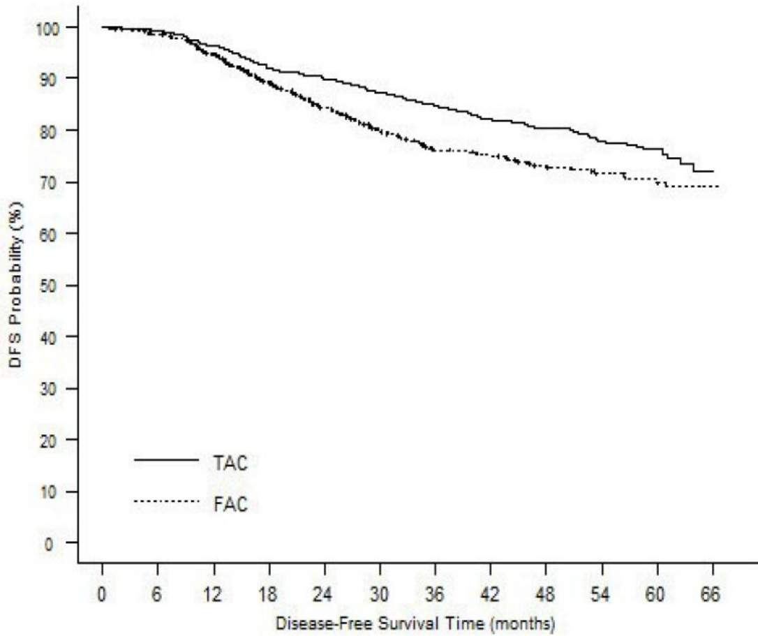
Figure 1: TAX316 Disease-Free Survival K-M curve
