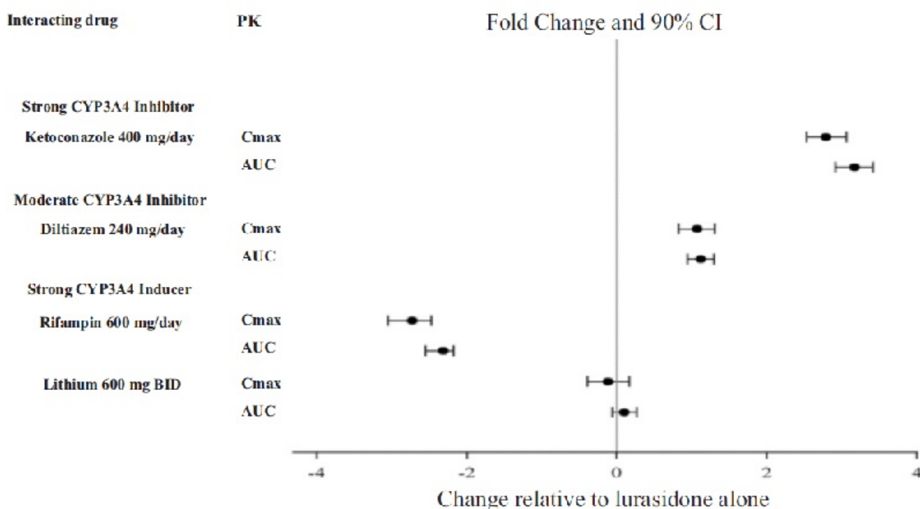
Figure 1: Impact of Other Drugs on Lurasidone Hydrochloride Pharmacokinetics
