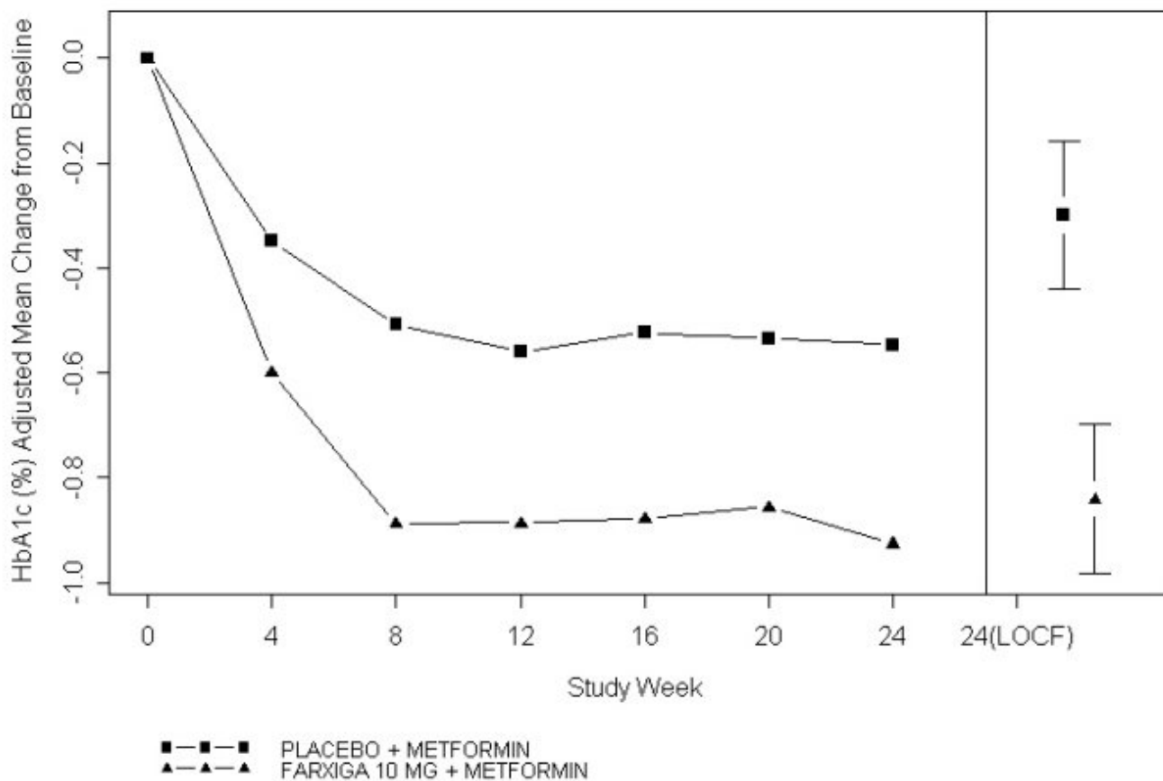
Left side graph: Values for adjusted mean change from baseline based on a longitudinal repeated measures model, including randomized subjects who completed Short-Term Period with both baseline and Week 24 HbA1c values without rescue. Right side graph for Week 24 (LOCF): Values for adjusted mean change from baseline and 95% CIs based on an ANCOVA model, including randomized subjects with a baseline and at least one post baseline HbA1c before rescue.
