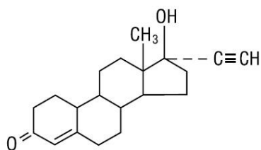
Norethindrone
