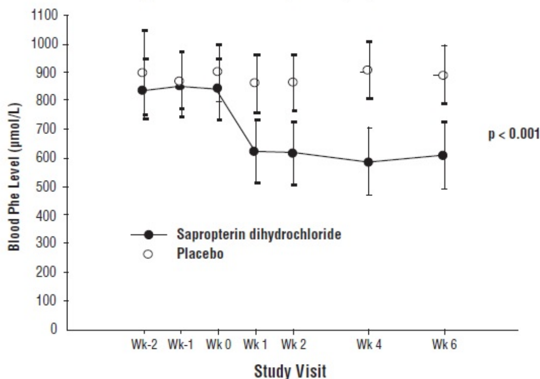
Figure 2: Mean Blood Phenylalanine (Phe) Level Over Time*
