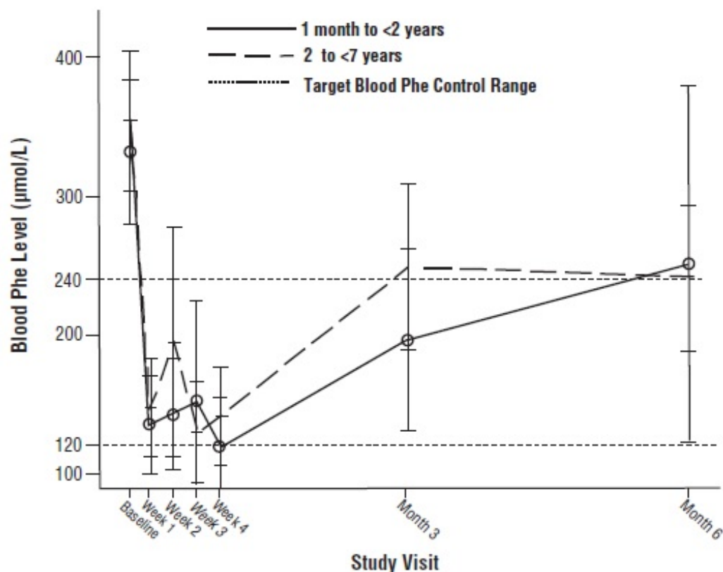
Figure 1: Mean Blood Phe Level Over Time by Age (years) (N=57)
