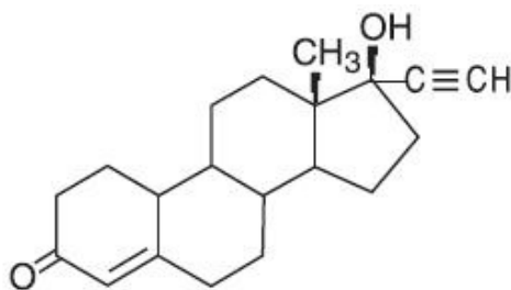
norethindrone
