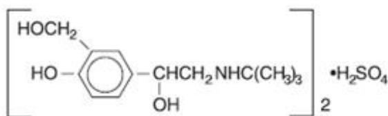
Figure 3.1-1. Chemical structure of albuterol sulfate.
