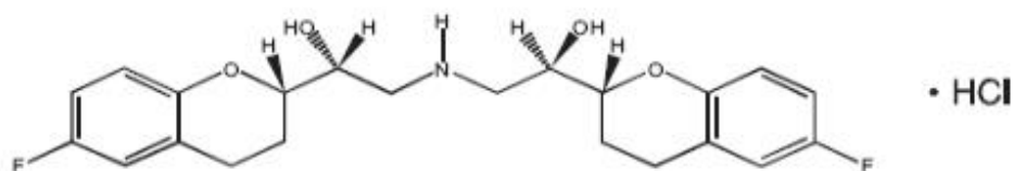
SRRR - or d-nebivolol hydrochloride
