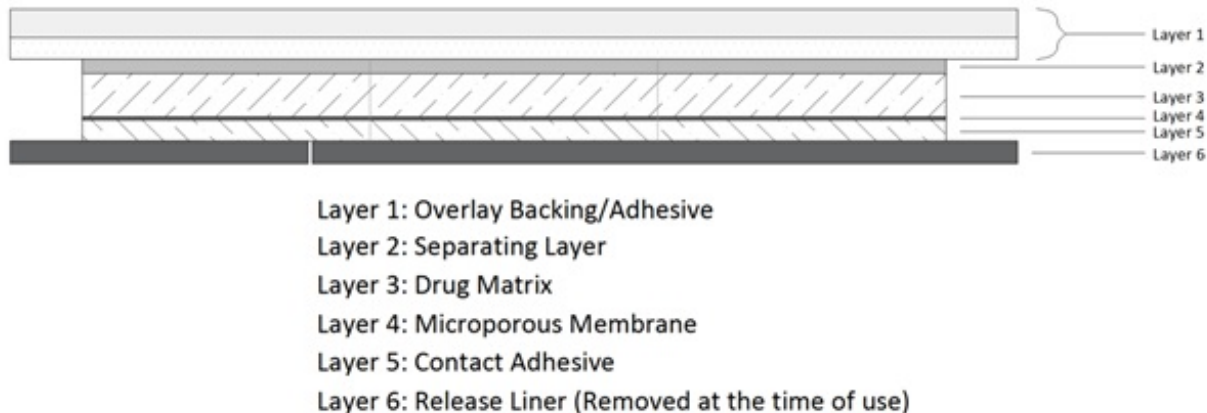
Figure 1: Cross Section of ADLARITY
