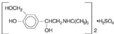
Figure 3.1-1. Chemical structure of albuterol sulfate.
