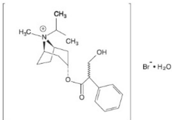
Figure 3.1-2. Chemical structure of ipratropium bromide.
