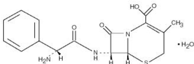
Structural Formula
