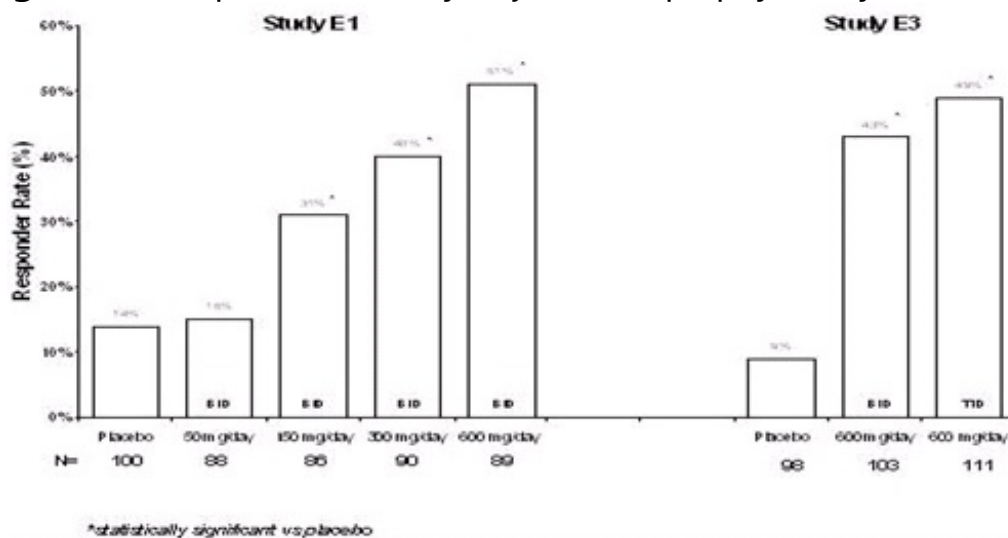
Figure 6: Responder Rate by Adjunctive Epilepsy Study
