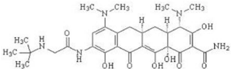
Figure 1: Structure of Tigecycline
