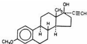
ethinyl estradiol Molecular formula C_{20}H_{24}O_2 M.W. = 296.41
