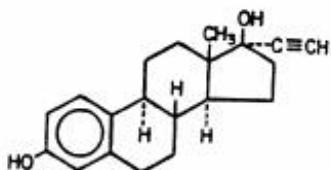
ethinyl estradiol Molecular formula C_{20}H_{24}O_2 M.W. = 296.41
