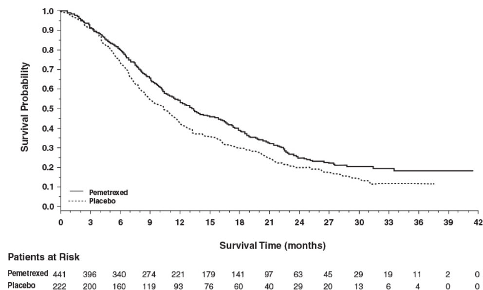
Figure 5: Kaplan-Meier Curves for Overall Survival in Study JMEN
