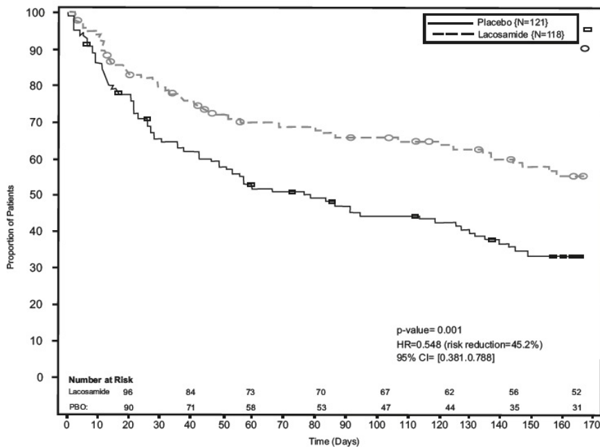
Figure 3 - Kaplan-Meier Analysis of Time to 2nd PGTC Seizure (Study 5) Analysis Set: Modified Full Analysis Set
