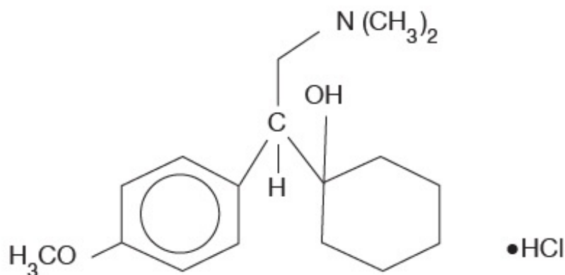
venlafaxine hydrochloride
