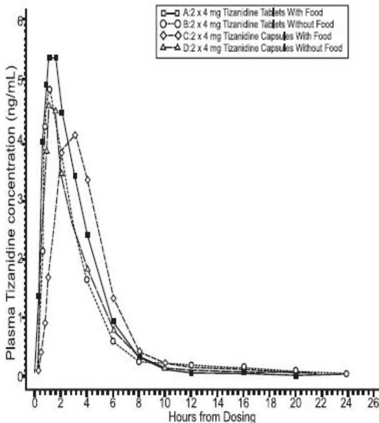
Figure 1: Mean Tizanidine Concentration vs. Time Profiles For Tizanidine Tablets and Capsules (2 × 4 mg) Under Fasted and Fed Conditions
