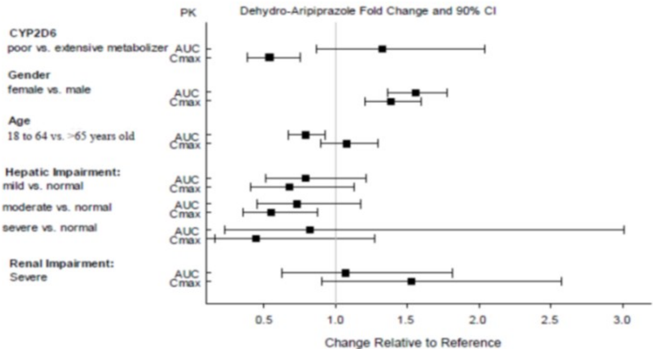
Figure 5: Effect of Intrinsic Factors on Dehydro-aripiprazole Pharmacokinetics
