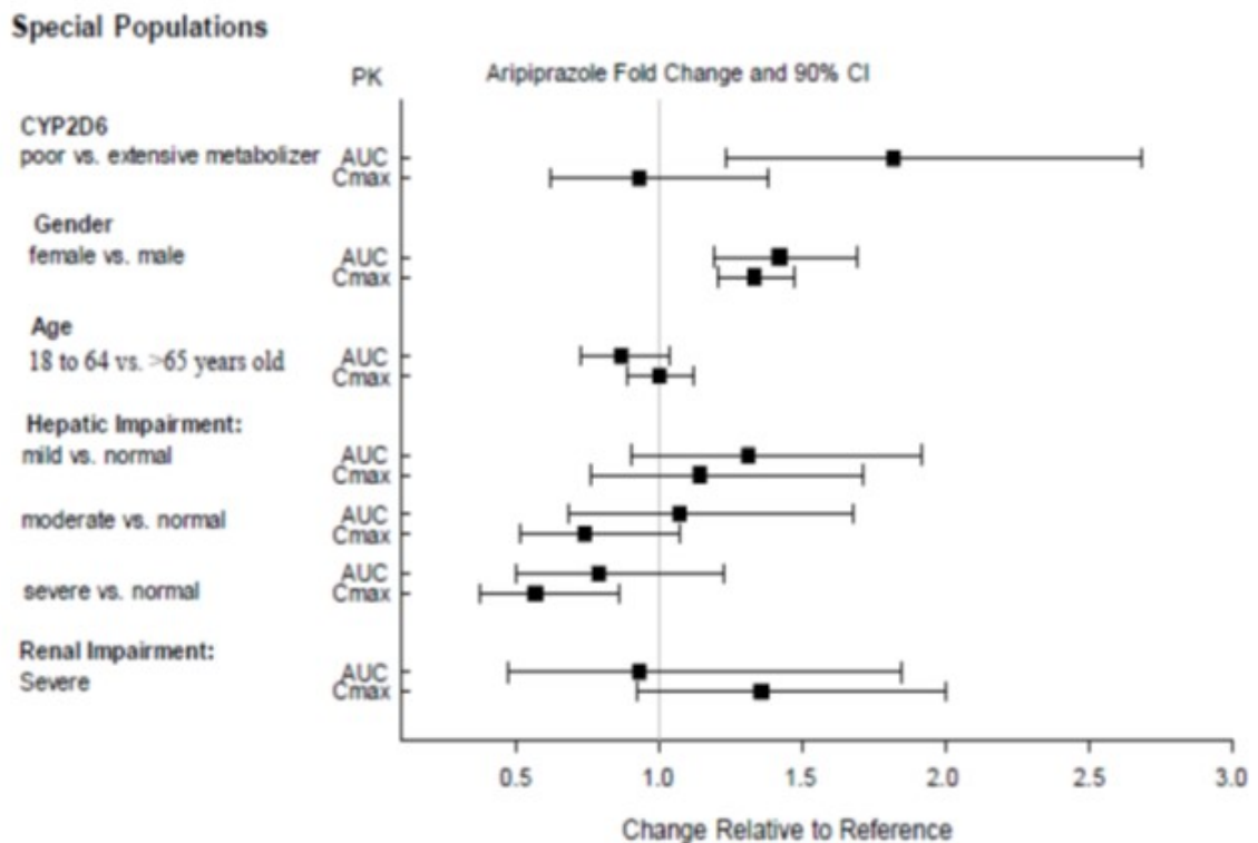
Figure 4: Effect of Intrinsic Factors on Aripiprazole Pharmacokinetics
