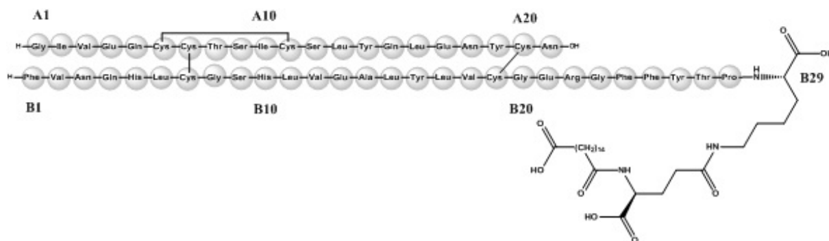
Figure 1: Structural Formula of TRESIBA
