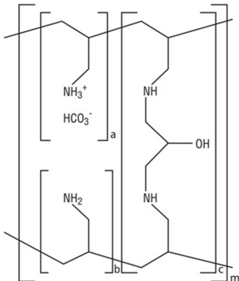
Figure 1. Chemical Structure of Sevelamer Carbonate
