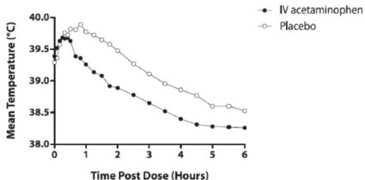
Figure 1: Mean Temperature (°C) Over Time
