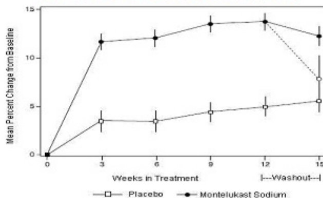
FIGURE 2: FEV 1 Mean Percent Change from Baseline (U.S. Trial: Montelukast Sodium N=406; Placebo N=270) (ANOVA Model)
