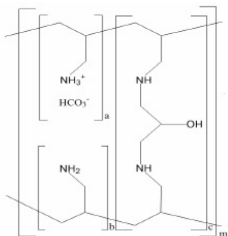
Figure 1: Chemical Structure of Sevelamer Carbonate
