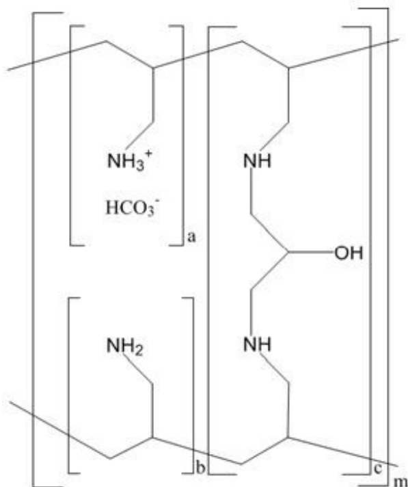
Figure 1: Chemical Structure of Sevelamer Carbonate
