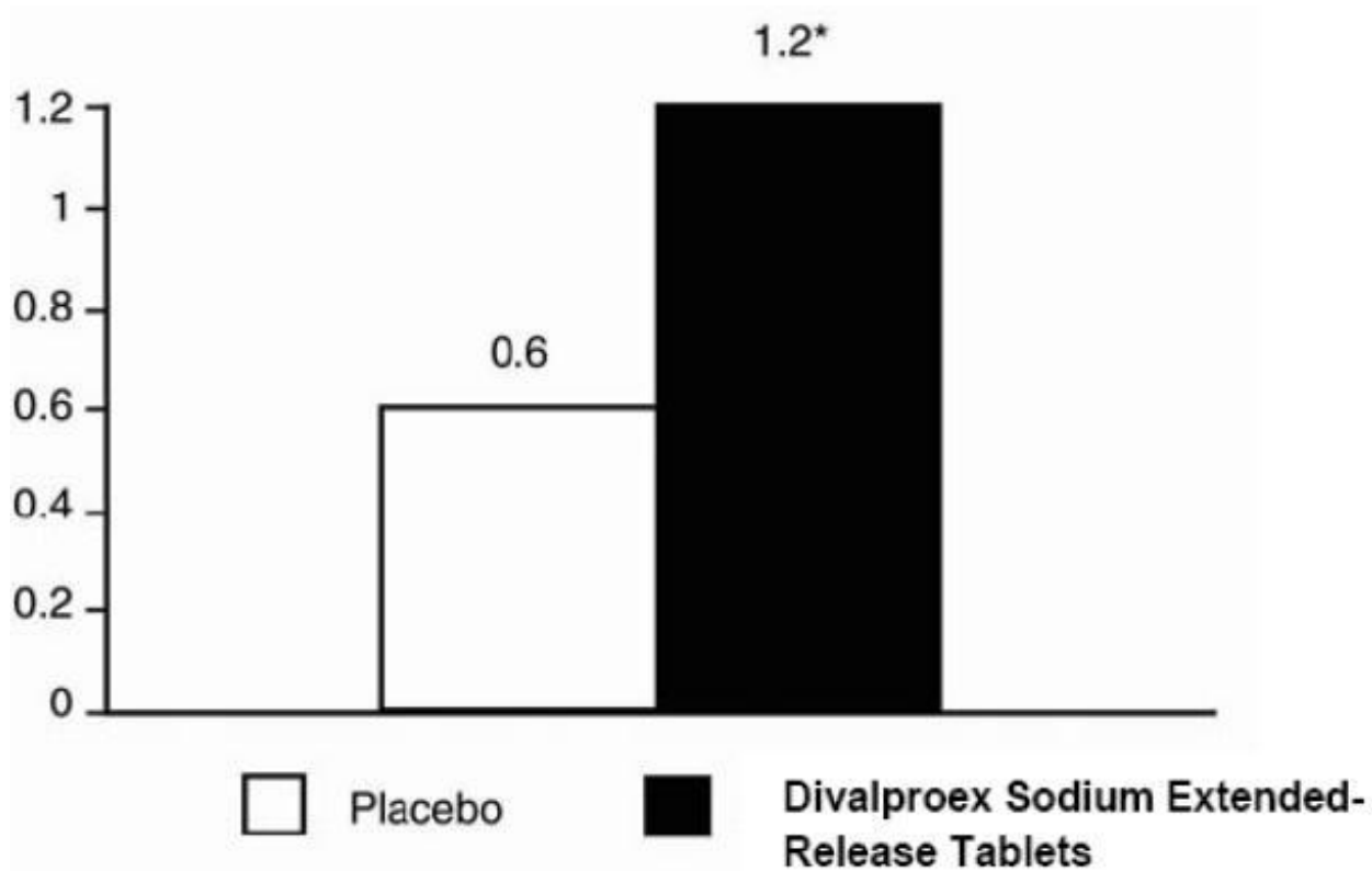
Figure 3. Mean Reduction In 4-Week Migraine Headache Rates
