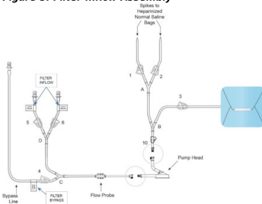
Figure 5: Filter Inflow Assembly
