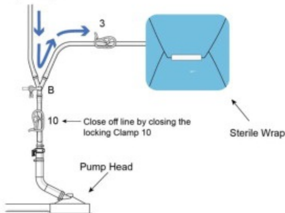
Figure 14: Prime Double Balloon Isolation Aspiration Catheter Line
