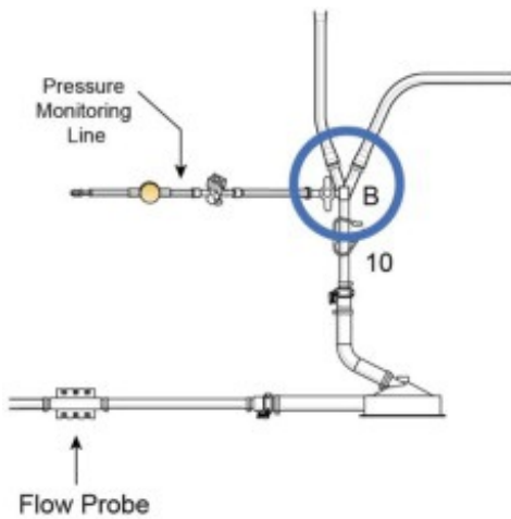
Figure 21: Attach and Prime Pre-Filter (Post-Pump) Pressure Line
