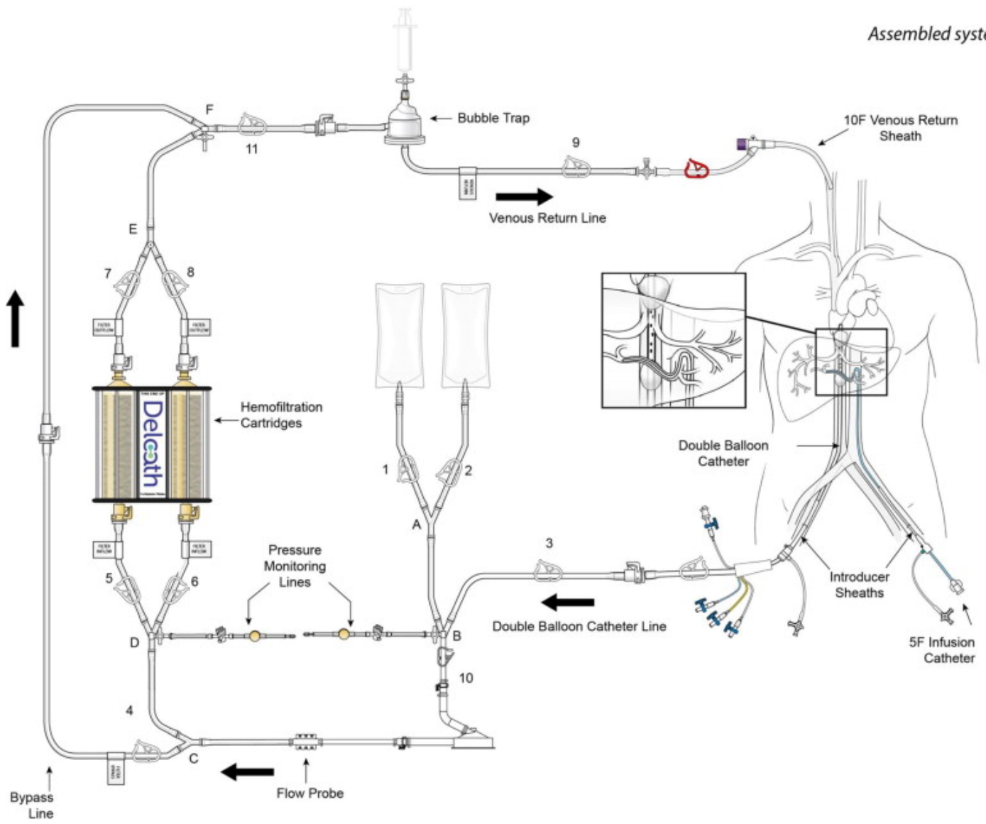
(b) SUPPLIED DISPOSABLE COMPONENTS - FIGURE 2
