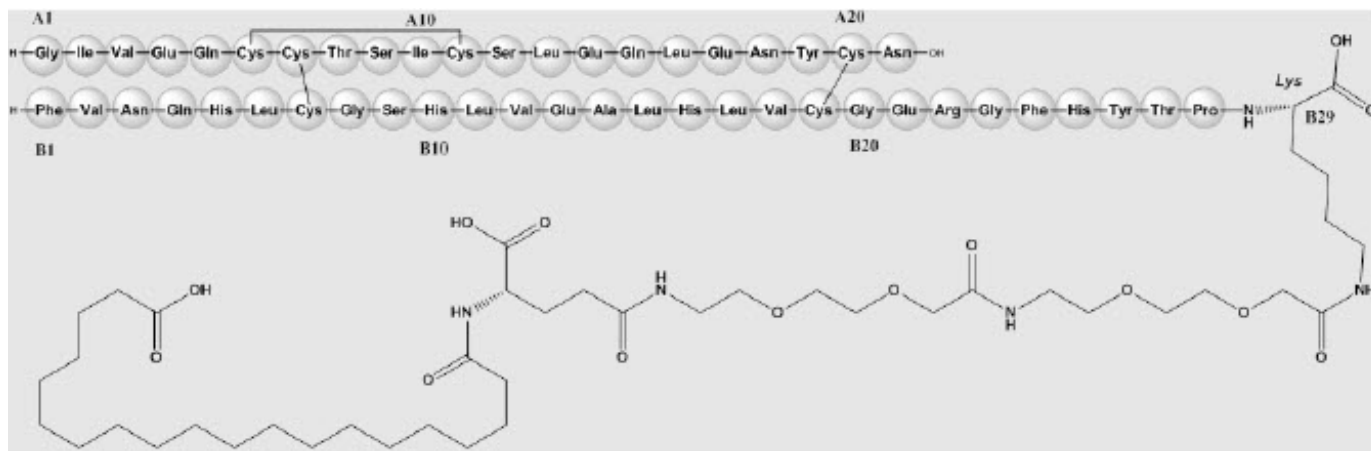
Figure 1: Structural Formula of Insulin icodec-abae
