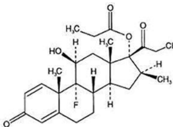
Clobetasol propionate
