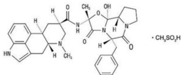
Dihydroergotamine Mesylate Structural Formula
