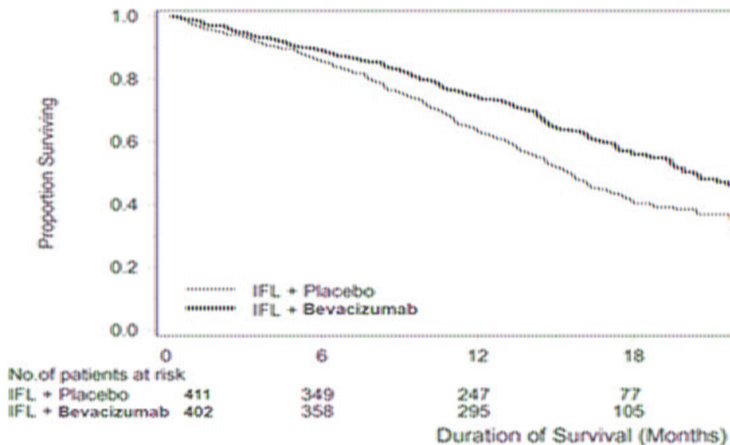
Figure 1: Kaplan-Meier Curves for Duration of Survival in Metastatic Colorectal Cancer in Study AVF2107g
