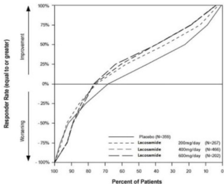
Figure 2 - Proportion of Patients by Responder Rate for Lacosamide and Placebo Groups in studies 2, 3 and 4
