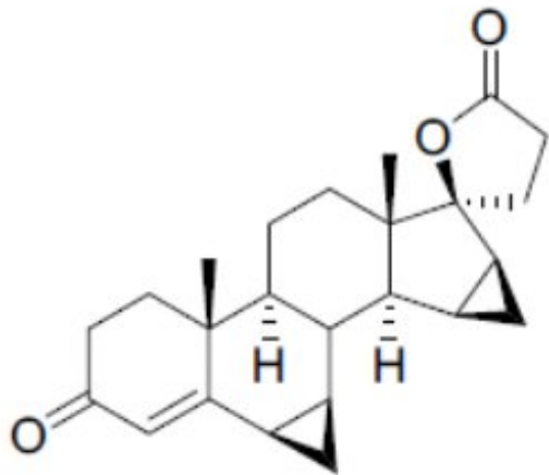
Drospirenone
