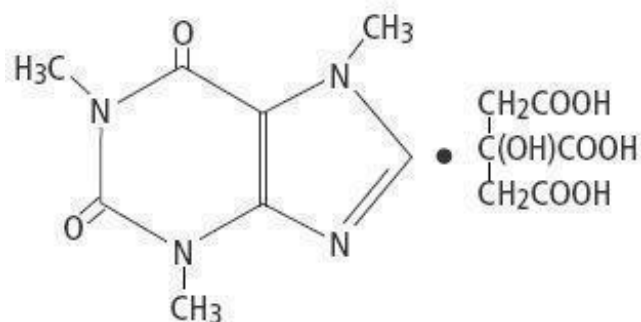
Caffeine citrate C_{14}H_{18}N_4O_9 Mol. Wt. 386.31
