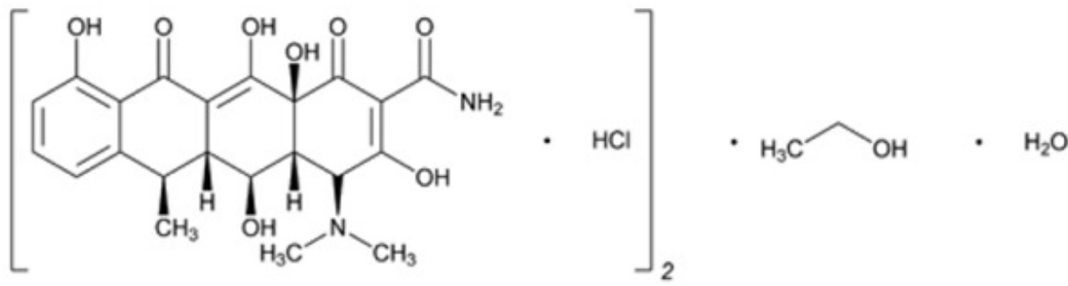
Figure 1: Structure of Doxycycline Hyclate
