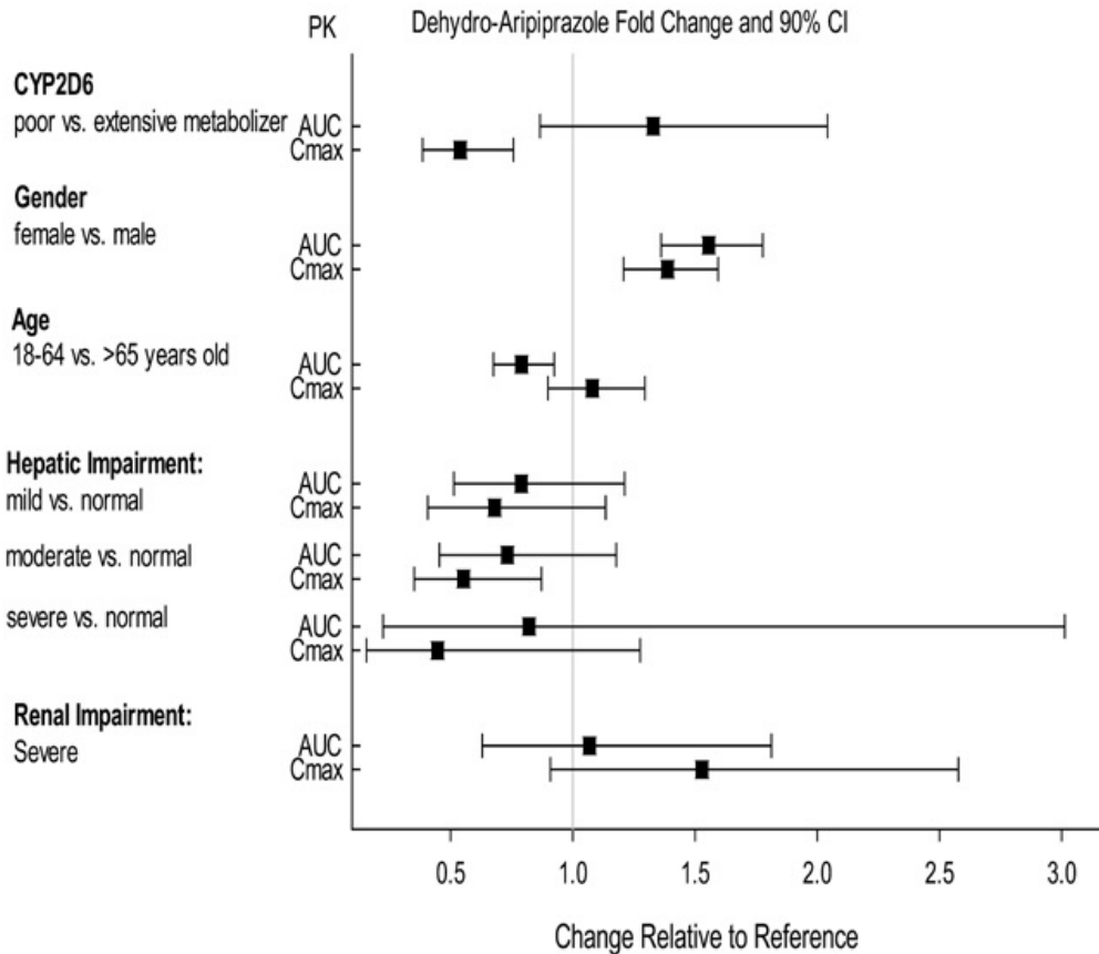
Figure 5: Effect of Intrinsic Factors on Dehydro-Aripiprazole Pharmacokinetics
