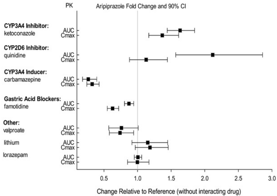
Figure 2: The Effect of Other Drugs on Dehydro-Aripiprazole Pharmacokinetics
