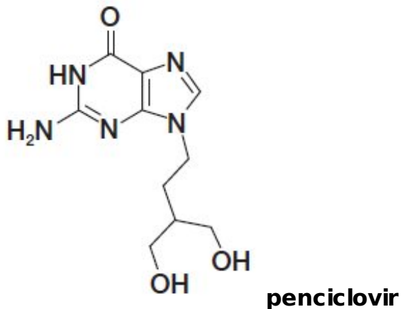
Figure 1: Structural Formula of Penciclovir
