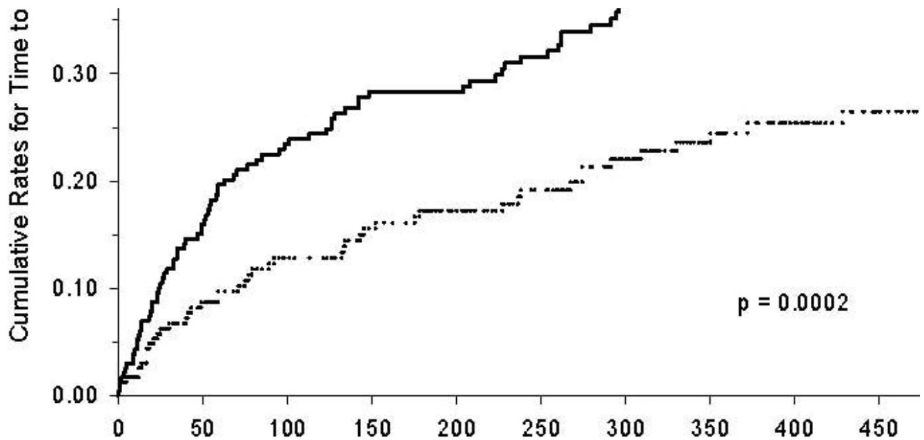
Figure 1: Kaplan-Meier Estimates of Cumulative Rates for Time to First Seizure
