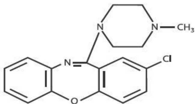
LOXAPINE BASE
