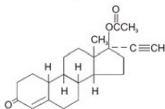
Norethindrone Acetate
