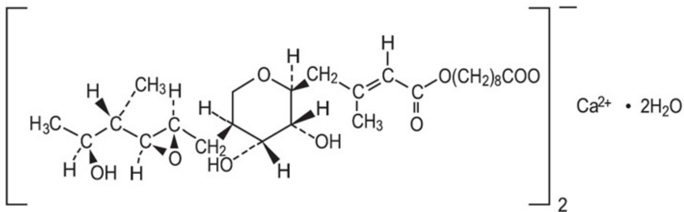
Figure 1. Structure of Mupirocin Calcium, USP
