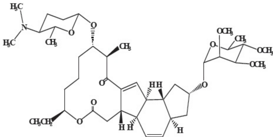
Spinosyn A(C 41 H 65 NO 10 ) MW731.461
