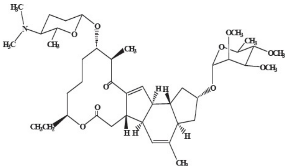
Spinosyn D(C 42 H 67 NO 10 ) MW745.477
