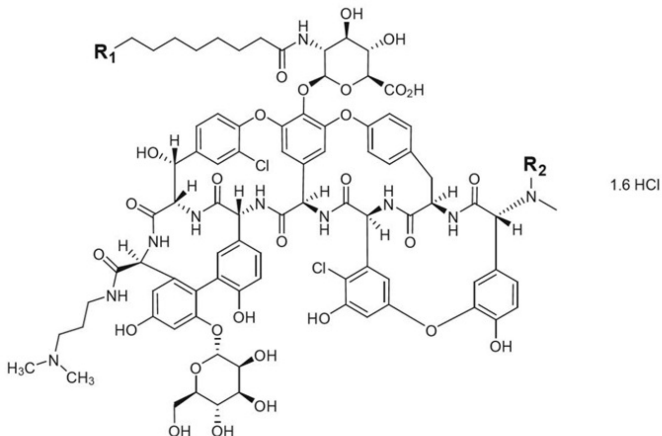
Figure 1. Dalbavancin Structural Formula
