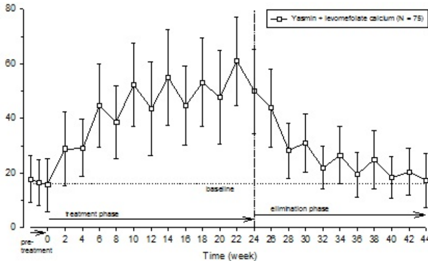
Figure 5: German Study: Mean trough concentration-time curve (and SD) of plasma folates after daily oral administration of Yasmin + levomefolate calcium
