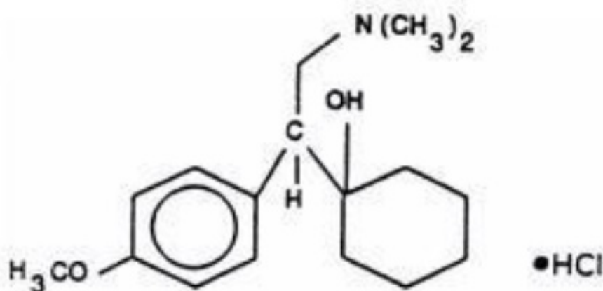
venlafaxine hydrochloride
