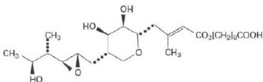
Figure 1. Structure of Mupirocin
