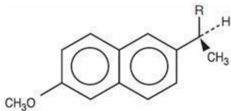
naproxen sodium (R=-COONa) C 14 H 13 NaO 3 mol wt 252.23
