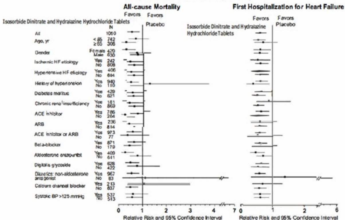
Figure 4: Results for Demographic, Baseline Medication and Clinical Characteristic Subgroups in Black Patients (A-HeFT)
