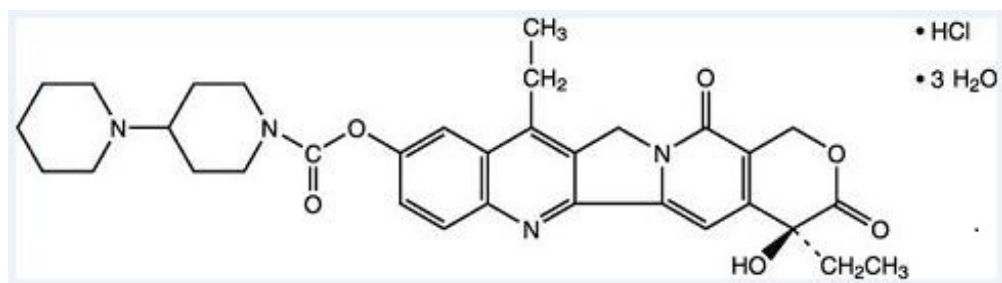
Irinotecan Hydrochloride
