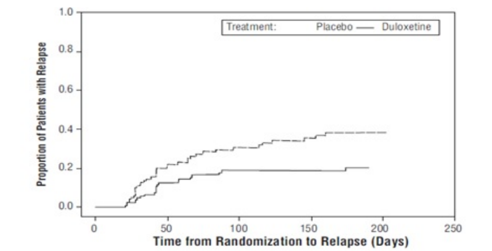
Figure 1: Cumulative Proportion a of Adult Patients with MDD Relapse (Study MDD-5)
